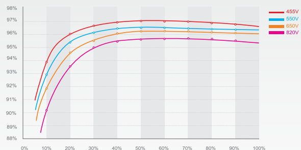
CP100 efficiency
